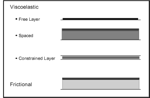
Fig2. Some viscoelastic material arrangements
