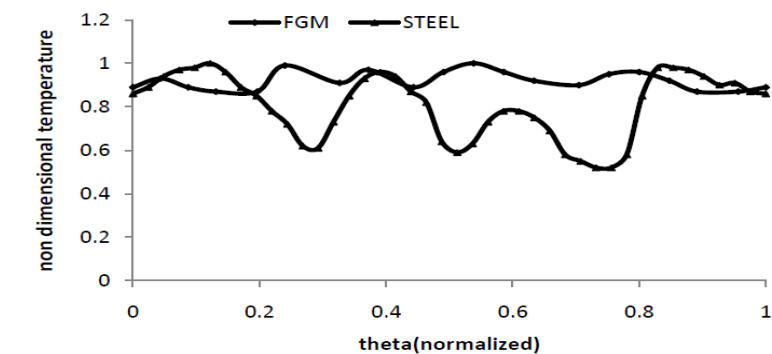
Fig5. normalized temperature distribution comparison between steel and FGM disk
