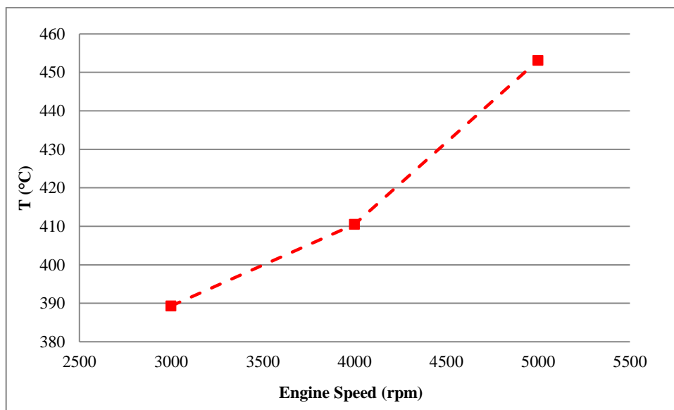
Fig.9. Steady State Exhaust Temperature
