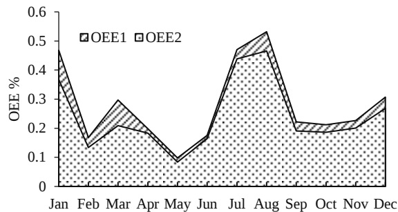
Figure 9. OEE_1 and OEE_2 metrics for Peugeot assembly line
