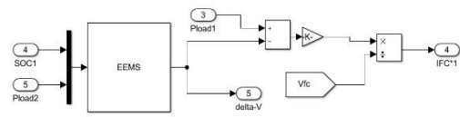
Fig.5. Energy management system: EEMS
