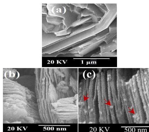
Figure 2. SEM images of (a) \text{Ti}_3\text{AlC}_2 MAX-phase, (b) \text{Ti}_3\text{C}_2\text{T}_x nano-sheets, (c) Super P/ \text{Ti}_3\text{C}_2\text{T}_x nano-composite.
