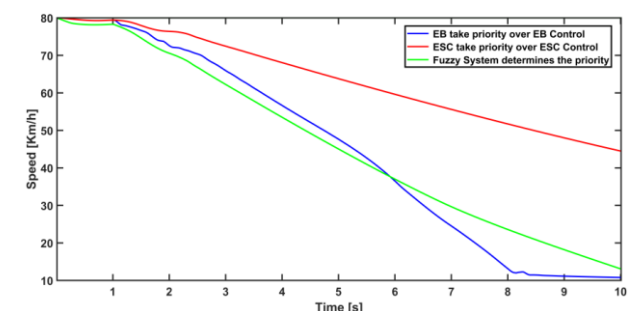
Figure 16. Vehicle speed in fishhook steering test
