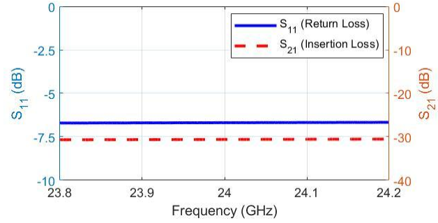
Figure 7. S-parameters during high-power limiting
