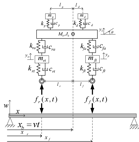
Fig. 5. The moving vehicle on a suspension bridge. Beam force interaction with a six DOF half-car planner model [6].
