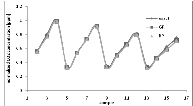
Fig9. Comparison of CO2 concentration predictions by GR and BP neural networks with experimental data for B10.
