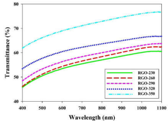
Fig. 3. Results of transmittance measurement of the RGO thin films.
