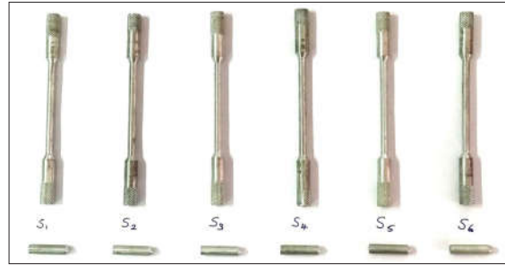
Fig. 3. Tensile and wear test samples
