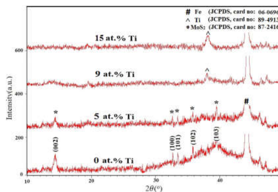
Fig. 8. XRD patterns of \text{MoS}_2 -Ti composite coatings with different Ti content.
