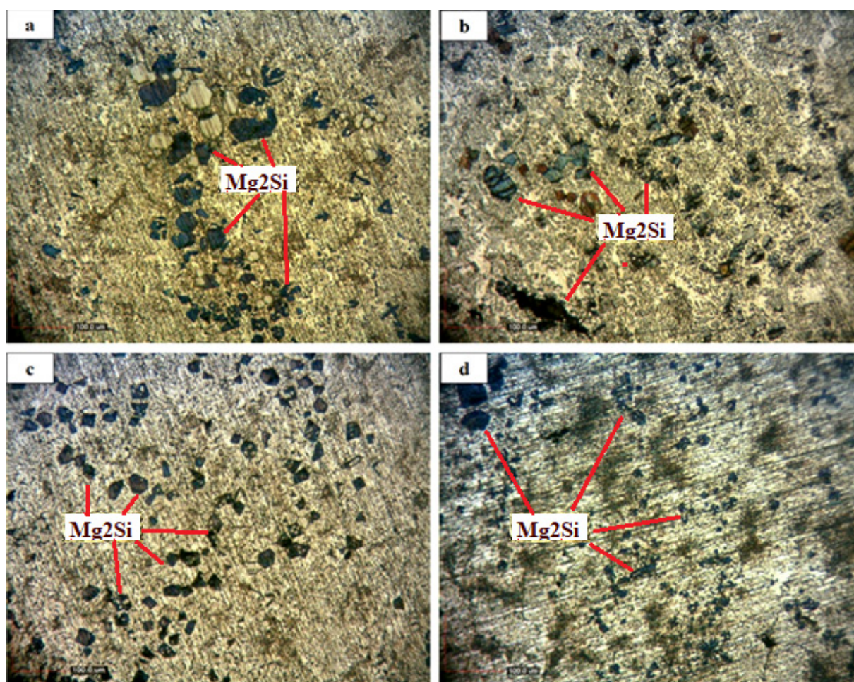
Fig. 6. Microstructures of 25% deformed after holding at 560°C for (a) 5 min, (b) 10 min, (c) 20 min and (d) 40 min for Al-15Mg 2 Si composite.
