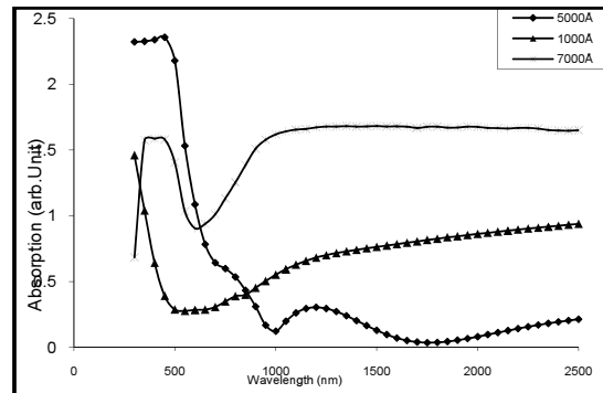
Fig. 6. Variation of absorbance spectra with wavelength for Cu 2 S films of different thicknesses
