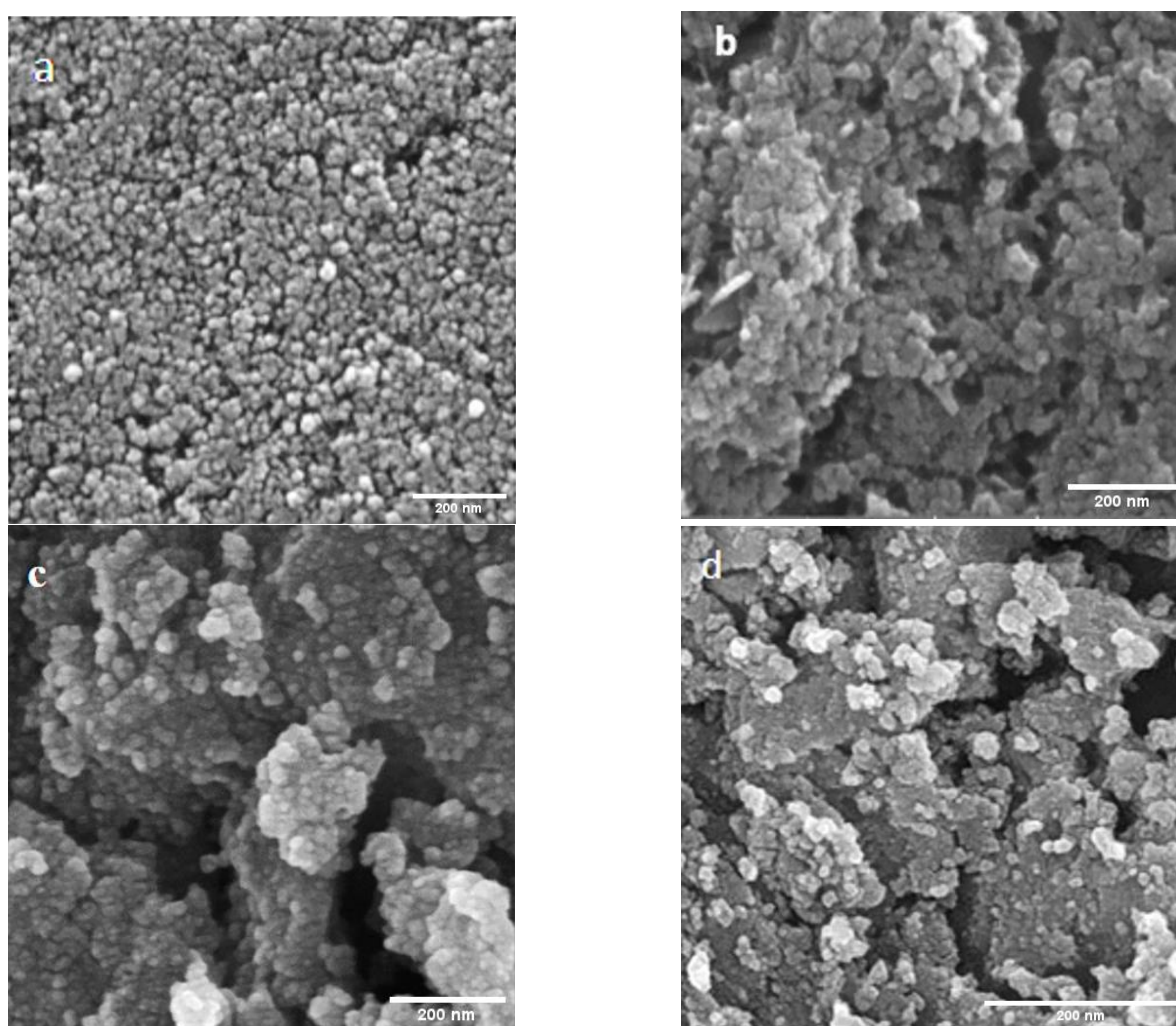
Fig. 3. FESEM image of a) \text{Fe}_3\text{O}_4 NPs synthesized with peppermint extract, b) \text{Fe}_3\text{O}_4 NPs without peppermint extract, c and d) \text{Fe}_3\text{O}_4@\text{m-SiO}_2 NPs
