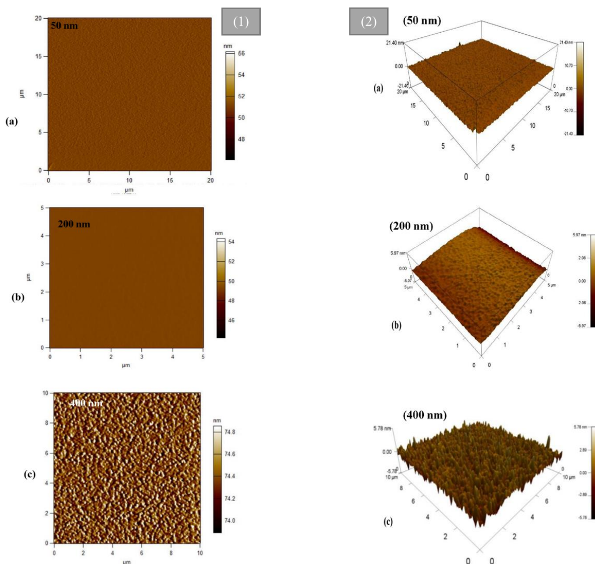
Fig. 8. (1) Specimen of 2D representative AFM images for a) 50 nm, b) 200 nm and c) 400 nm thin films. Scan area: 20 \mu\text{m} \times 20 \mu\text{m} , 5 \mu\text{m} \times 5 \mu\text{m} , 10 \mu\text{m} \times 10 \mu\text{m} (2) Specimen of 3D representative AFM images for a) 50 nm, b) 200 nm and c) 400 nm thin films. Scan area: 20 \mu\text{m} \times 20 \mu\text{m} , 5 \mu\text{m} \times 5 \mu\text{m} , 10 \mu\text{m} \times 10 \mu\text{m}
