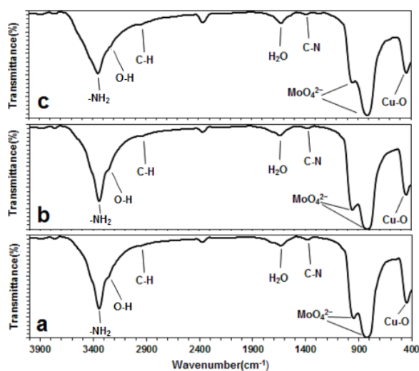
Fig. 2. Infrared spectra of the as-prepared colloidal \text{Cu}_3(\text{MoO}_4)_2(\text{OH})_2 with various architectures: a) rod, b) sheet and c) hollow sphere morphology
