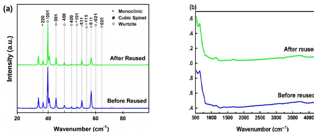
Fig. 15. a) XRD patterns of \text{Fe}_3\text{O}_4/\text{ZnO}/\text{CuO} nanocomposites before reused, b) IR peaks of \text{Fe}_3\text{O}_4/\text{ZnO}/\text{CuO} nanocomposites after and before reused [30]
