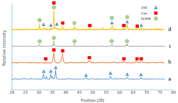
Fig. 1. XRD patterns of synthesized \text{Fe}_3\text{O}_4/\text{ZnO}/\text{CuO} nanocomposite: a) ZnO, b) CuO, c) \text{Fe}_3\text{O}_4 , d) \text{Fe}_3\text{O}_4/\text{ZnO}/\text{CuO} nanocomposite
