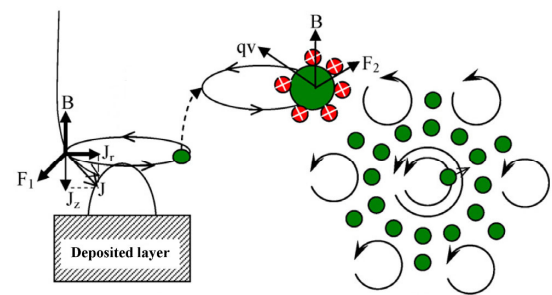
Fig. 2. Schematic diagram of the current vectors around the particles [16].
