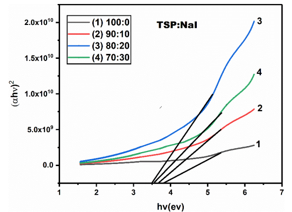
Fig. 9. ‘Direct allowed energy bandgap’ plot for different wt.% ratios of TSP-NaI
