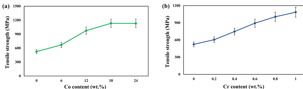
Fig. 8. Tensile strength values of the cermets consisting of various binder contents: a) WC-Co and b) WC-Cr
