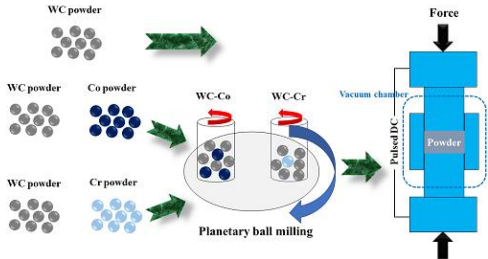
Fig. 2. A schematic demonstration of the ball milling and SPS processes applied in the present work
