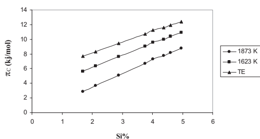
Fig. 3. Effect of silicon percent on the graphitization potential in 1873 K, 1623 K and eutectic transformation temperatures in (Fe- G) system of alloys
