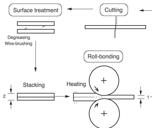
Fig. 1. Schematic illustration showing the principle of the accumulative roll bonding (ARB) [22].
