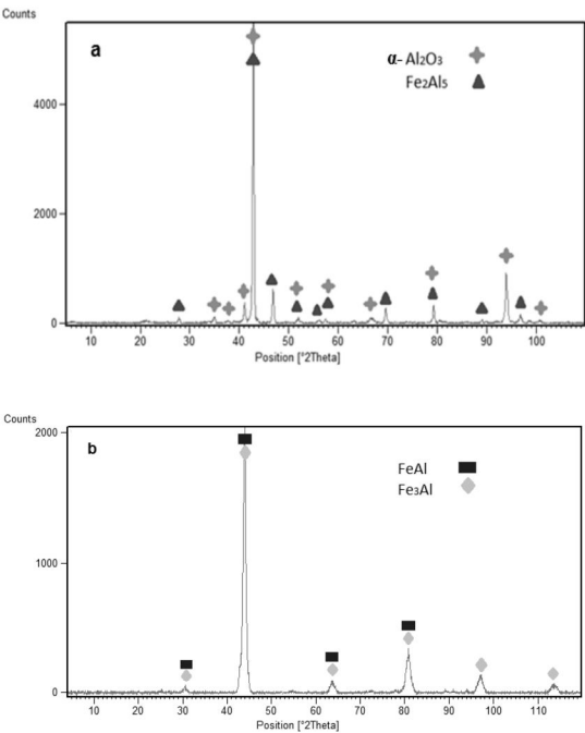
Fig. 3. XRD pattern of specimen aluminized at 750 °C for 4 minutes and heat treated at 1000 °C for 20 minutes. a) Sample surface, b) surface of the sample after removal a 100 µm layer from the surface by machining.
