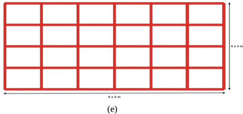
Figure 9. The 10-story with 1026-Member steel frame, (a) 3-D view (b) side view of frames 2, 3 and 4 (c) side view of frames 1 and 5 (d) side view of frames A, B, C, D, E, F and G (e) plan view
