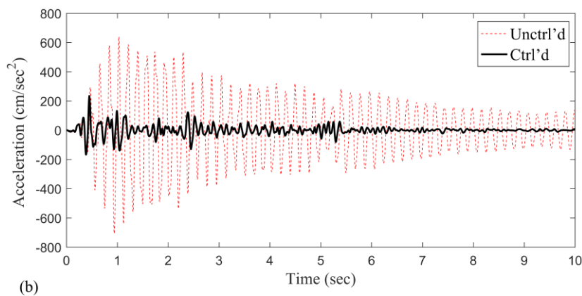
Figure 8. Time histories of responses on the third floor under the low (50%) El Centro earthquake: (a) drift; and (b) acceleration
