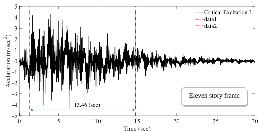
Figure 1: The acceleration time history for critical excitations for different concrete moment frames
