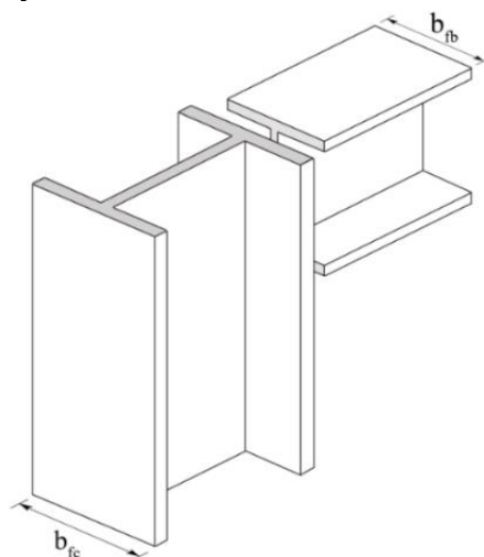
Figure 4: beam-to-column connection
