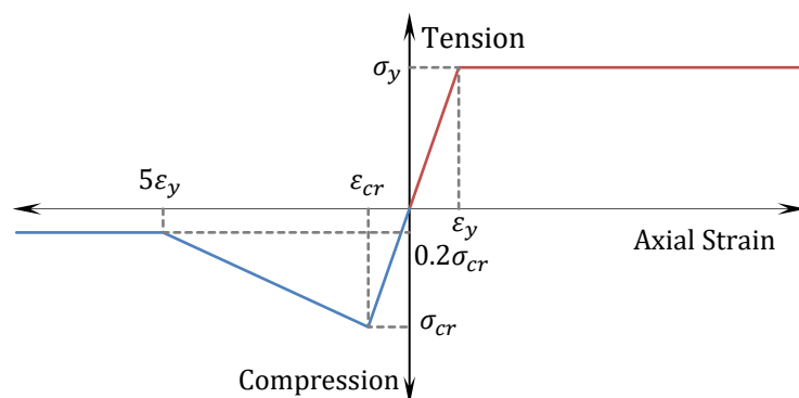
Figure 2: Stress-Strain Curve of Brace Behavior
