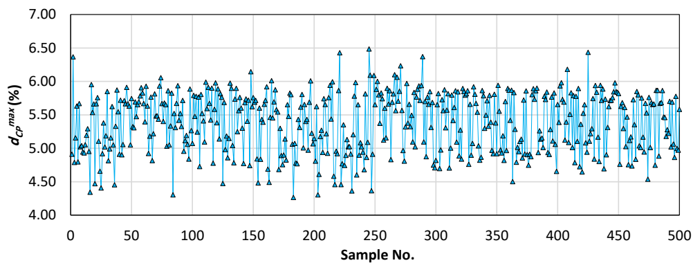
Figure 17: Maximum inter-story drift ratios at the CP level for the 12-story frame
