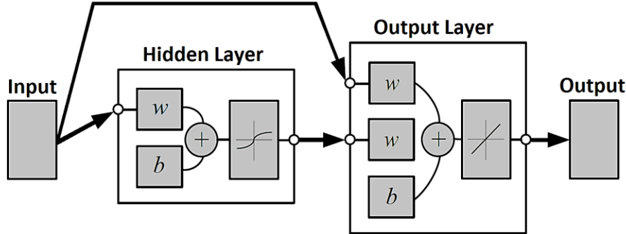
Figure 3: CFBP neural network model
